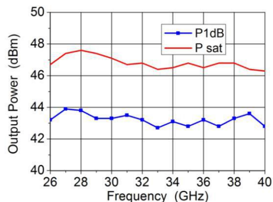
S3871FF Output power VS Frequency
