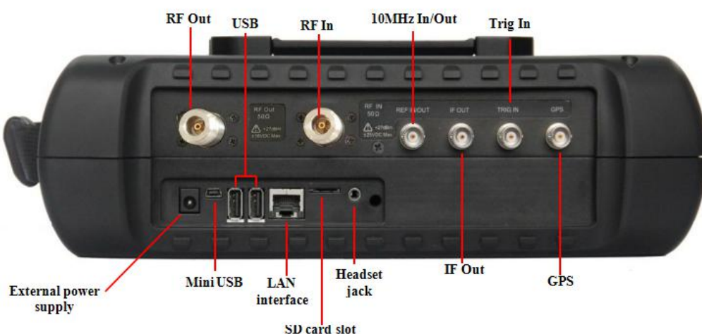
Fig. 3-3 Interface Description
