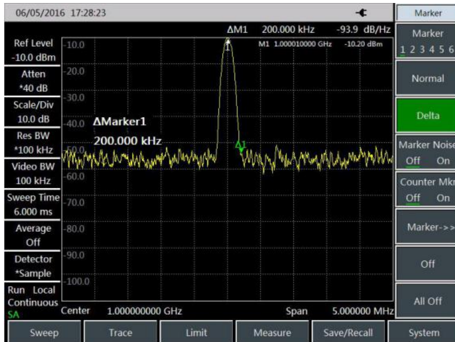
Fig. 4-10 S/N Measurement
